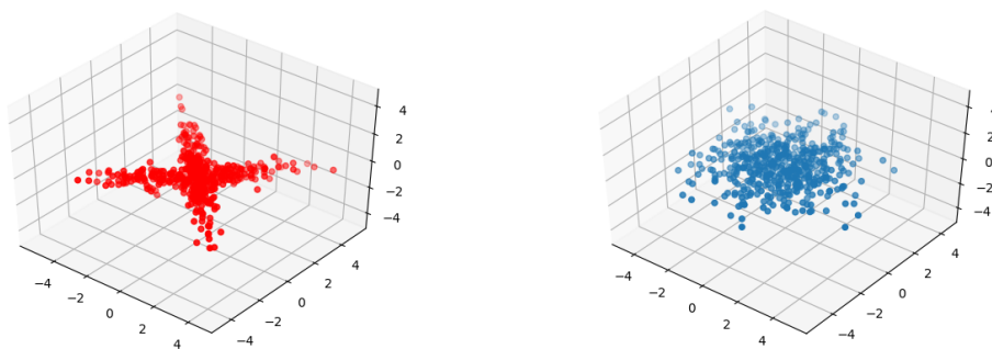
Figure 20.1: PCA cannot distinguish between the situations depicted in the two datasets.
